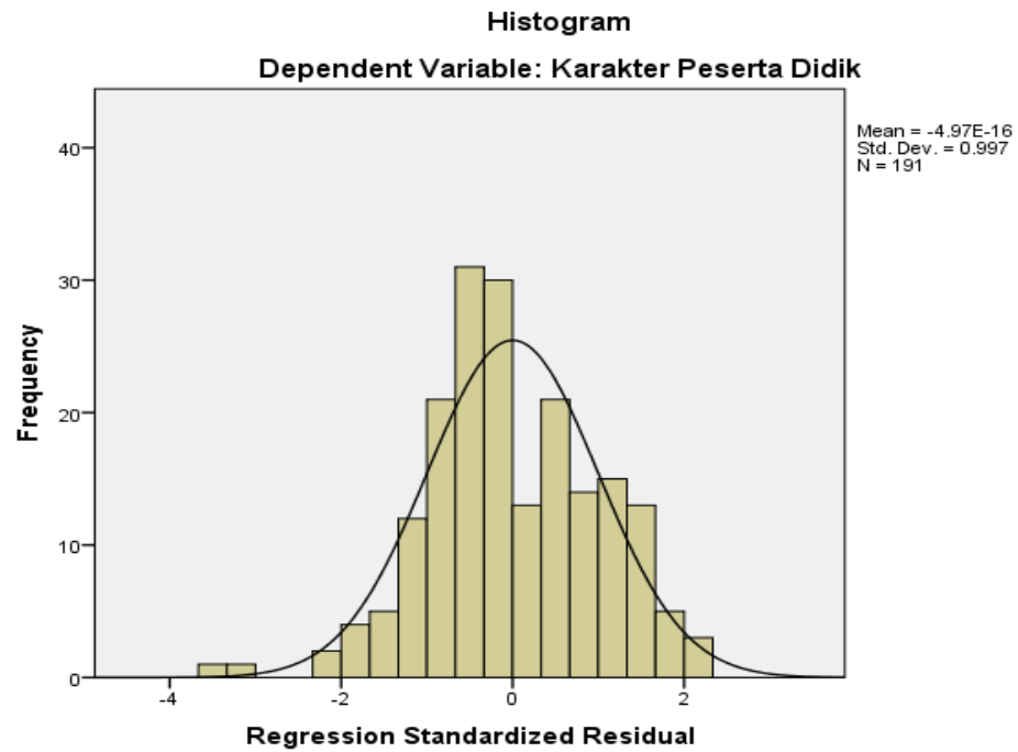
Gambar 4.3 Histogram Berdistribusi Normal
