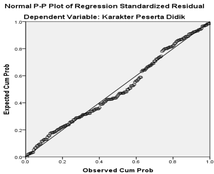
Gambar 4.4 P-Plot Berdistribusi Normal
